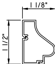
1 1/8"X1 1/2" SNAP TRIM M22378 - BASE CLIP M22438 - TRIM
