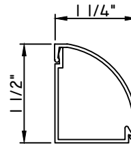
1 1/4"X1 1/2" SNAP TRIM M15266 - BASE CLIP M17164 - TRIM
