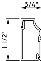
3/4"X1 1/2" SNAP TRIM M2144 - BASE CLIP M2143 - TRIM
